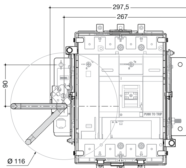
Drawout system x630
