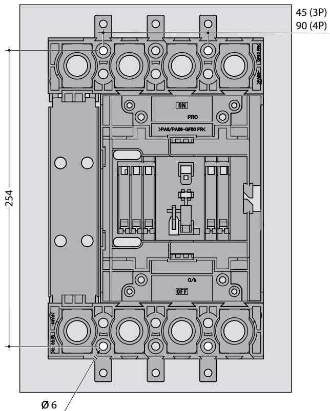
P630 circuit breaker on plug-in kit
