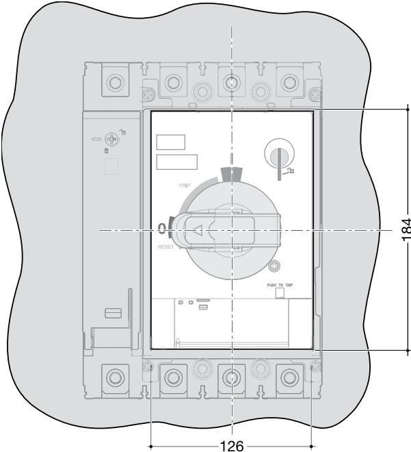
66_Panel_cut-out_rot_han_x630_4P
